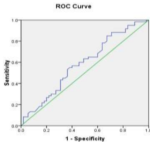
Figure 2. Graphic ROC
